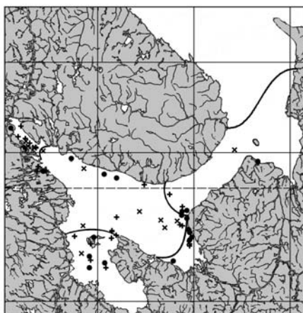
18. Lyonsia arenosa
