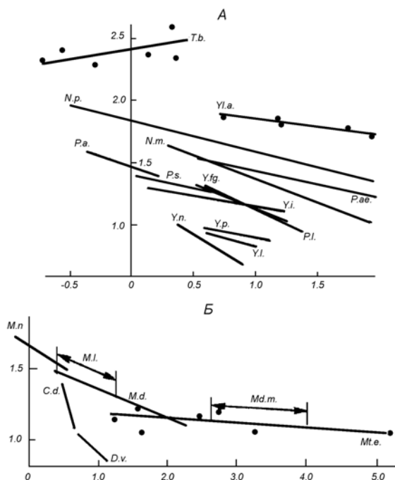
Fig. 8. Relationship between a_3 and R_3 statistics. X-axes – absolute term a_3 , Y-axes – coefficient of regression R_3 . Notations as in figures 6 and 7. Points are displayed only for Yoldia hyperborea , Tridonta borealis (A) and Mytilus edulis (B). After Naumov, Fedyakov, 1985, z.
