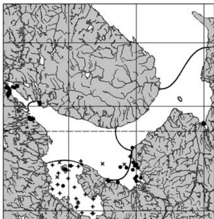
35. Arctica islandica
