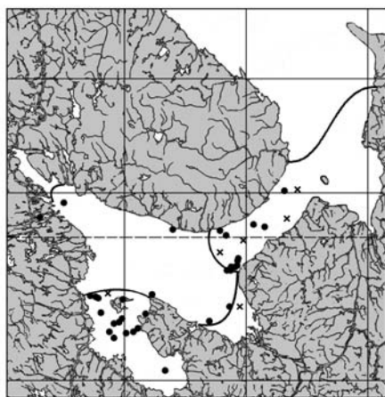
3. Nuculana minuta
