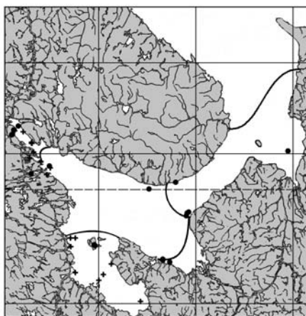
8. Musculus discors
