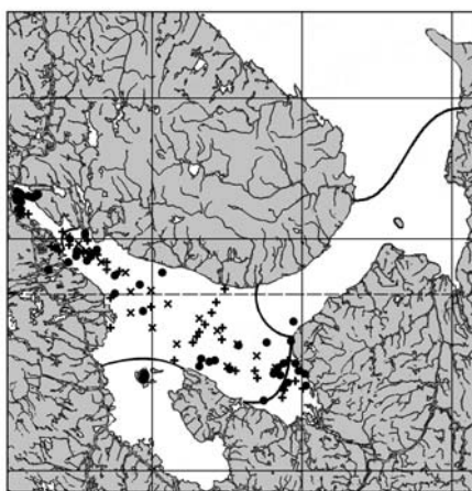
4. Portlandia arctica
