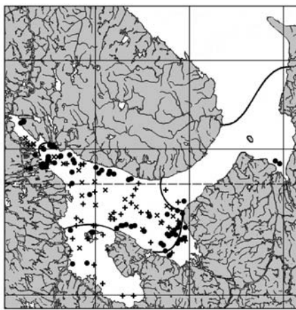
2. Nuculana pernula
