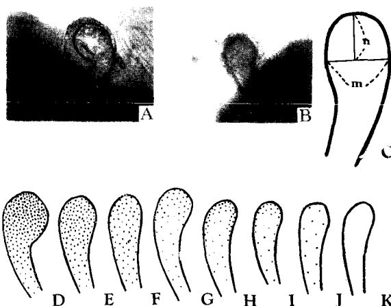
Fig. 4. Spermatheca. A & B. Photomicrographs (photo by Mr. H. Nakahara). \times 70 . A. E. pustulosa , PI. B. E. vigintioctomaculata , VI. C. Showing the method of measuring the apical index, S. m/n \sim S . D-K. Showing the scala of the coloration of spermatheca (Schematic). D. Dark brown. E. Moderate brown. F. Pale brown. G, H & I. Apex and margin alone showing various shades of brown, other parts yellowish or typically white. J. Yellowish white. K. Typically white.
