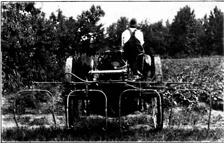
FIGURE 28.—Power sprayer, showing proper arrangement of the boom and nozzles for spraying the undersurfaces and tops of the leaves (N. F. Howard).
