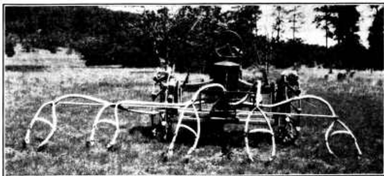
FIGURE 26.—Power duster mounted on tractor for rapid dusting. Note arrangement of nozzles, two per row. Nozzles made from tin grocery scoops and clamped to distributor pipe with automobile hose connections.
