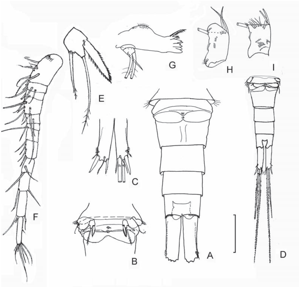
Fig. 2. Eucyclops romaniensis sp. nov. A – abdomen, dorsally, B – genital double somite, ventrally; C – caudal rami dorsally; E – rudimentary leg 5; F – antenna; G – mandible; H, I – posterior and anterior sides of antennal base. Scale bar: 100 \mu m (A–C), 75 \mu m (E–F), 50 \mu m (D, G–H).
