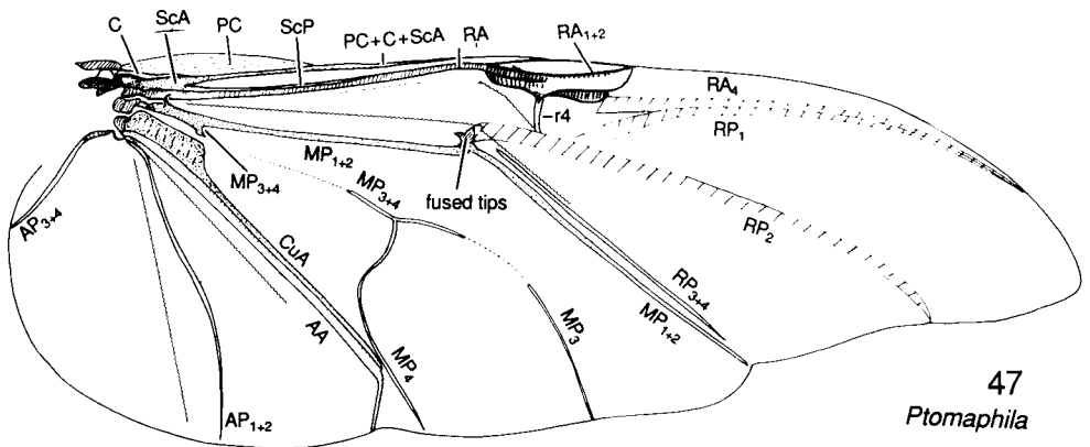
FIGS. 45-47. Staphylinoidea: 45, Necrophilus hydrophiloides Mannerheim (Agyrtidae); 46, Creophilus erythrocephalus (Fabricius) (Staphylinidae); 47, Ptomaphila lacrymosa (Schreibers) (Silphidae).
