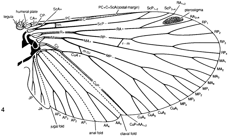
FIGS. 3-4. 3, scheme of pterygote wing venation, with articulation, complete veinal system, folds, venational braces, and veinal fusions; the ancestral band of unused sclerites (P = proxalare, AX = axalare, F = fulcalare, B = basivenale) gave rise to all Recent types of wing articulation (after Kukulová-Peck 1983); 4, generalized Neoptera wing venation (after Lawrence et al. 1991).
