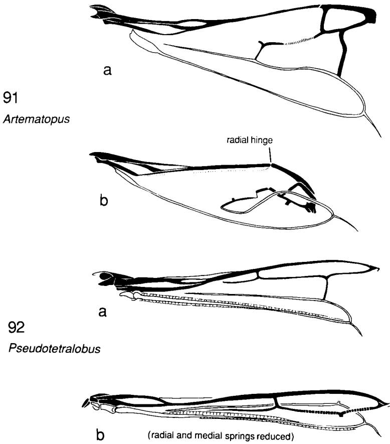
FIGS. 91-92. The positions of the radial and medial loops in the unfolded (a) and folded (b) wings: 91, Artematopus sp. (Artematopidae); 92, Pseudotetralobus sp. (Elateridae).
