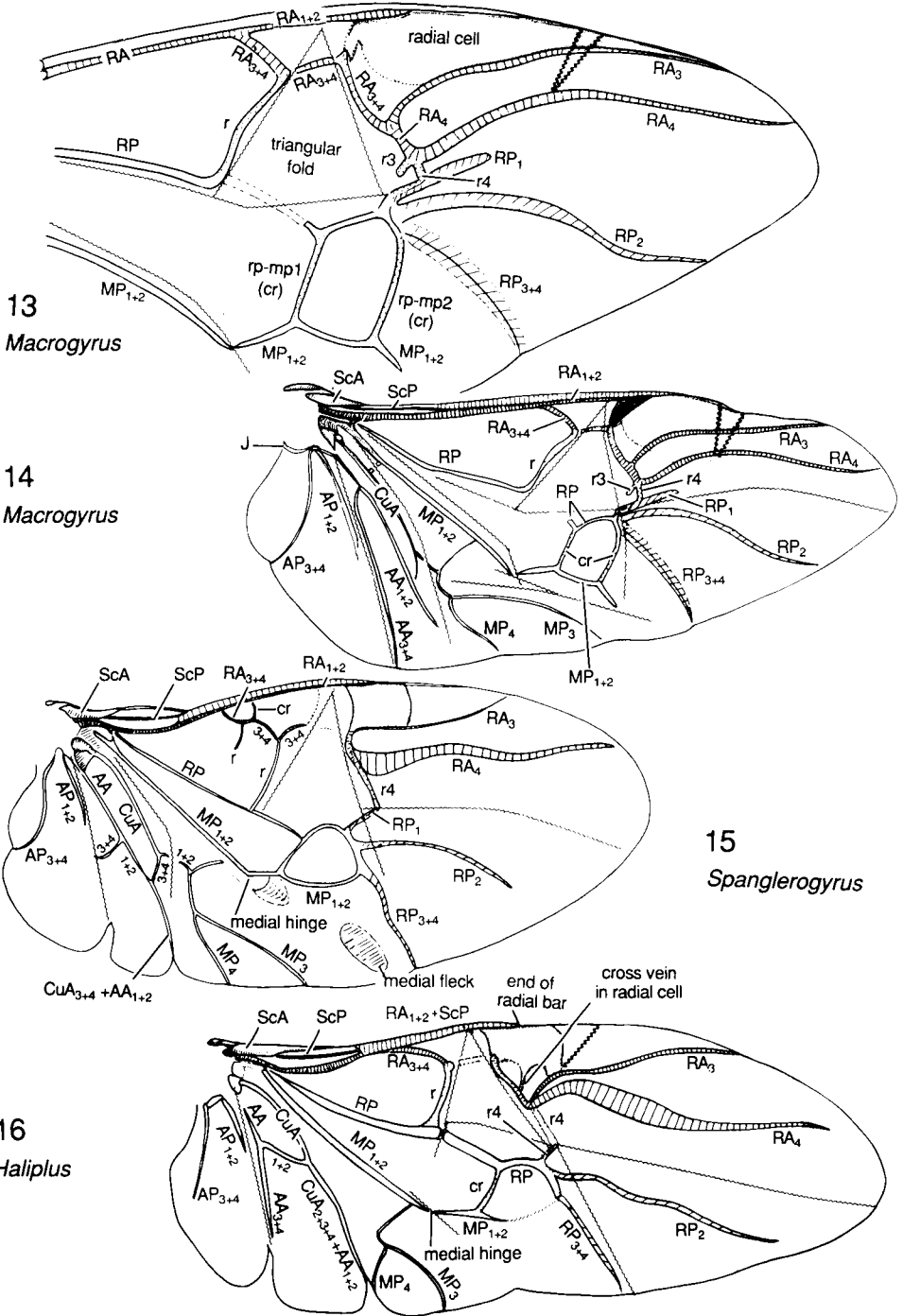
FIGS. 13-16. ADEPHAGA: 13-15, GYRINIDAE: 13, Macrogyrus sp., apical region only; 14, Macrogyrus sp.; 15, Spanglerogyrus albiventris Folkerts; 16, HALIPLIDAE: Halipilus bistriatus Wehncke.
