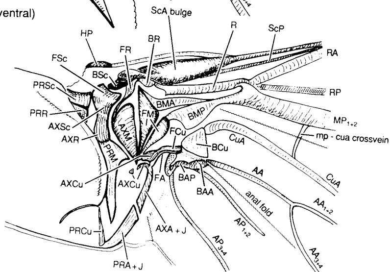
FIGS. 72-73. Axillary region and wing base of Adephaga, Macrogyrus sp. (Gyrinidae): 72, ventral, showing basalare, subalare, and part of attached metapleuron (composite, semi-diagrammatic); 73, dorsal, showing part of metatergum.
