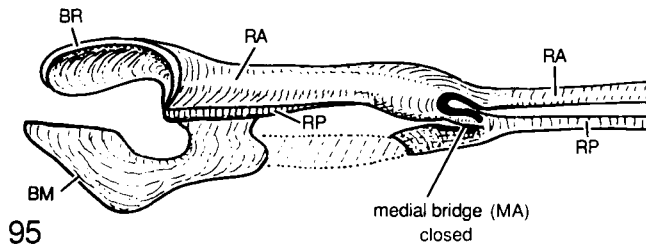
FIGS. 93-95. Bases of the radial and median veins and medial bridge in hind wing of Priacma serrata (LeConte): 93, extended wing, showing open, V-shaped medial bridge; 94, same, ventral, showing base of RP lying beneath bridge and RA; 95, folded wing, showing closed, U-shaped bridge.
