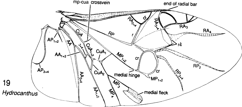
Figs. 17-19. Adephaga: 17, Trachypachus gibbsi LeConte (Trachypachidae), detail of anterior wing base; 18, Hygrobia nigra (Clark) (Hygrobiiidae); 19, Hydrocanthus australasiae Wehncke (Noteridae).
