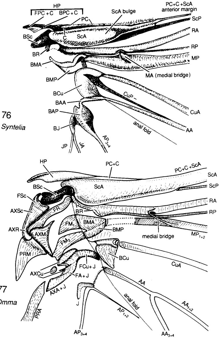
Figs. 76-77. Axillary region and wing base of Archostemata: 76, Syntelia mexicana Westwood (Synteliidae); 77, Omnia stanleyi Newman (Ommatidae).
