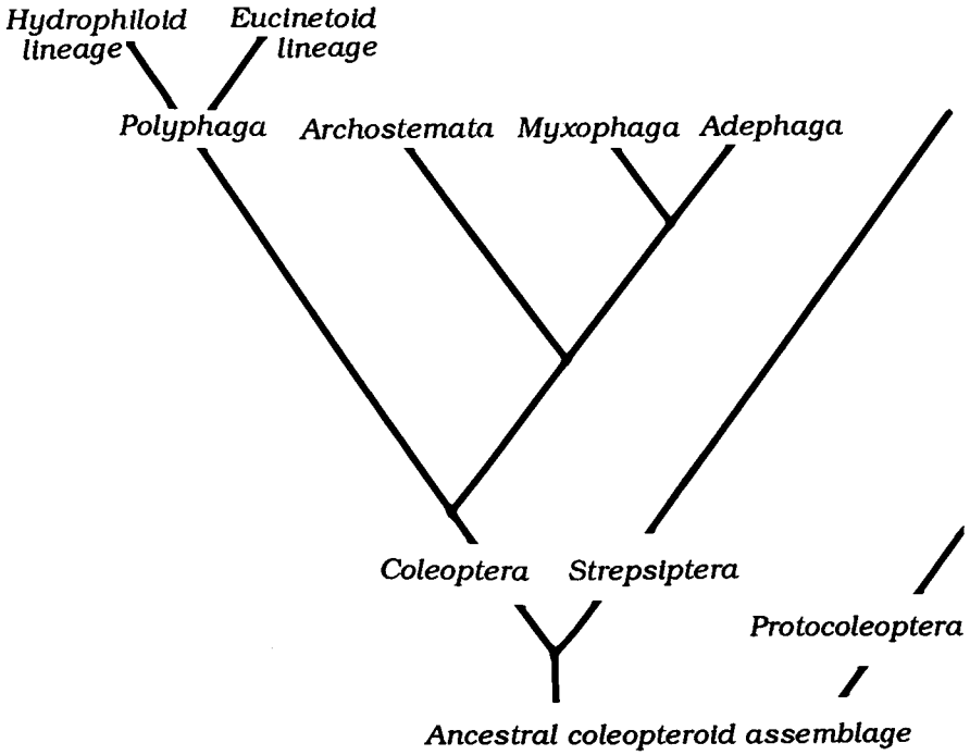
FIG. 102. Summary diagram of the phylogenetic relationships of the major groups of the coleopteroid assemblage. Data on the apomorphies that define the clades are given in the text.
