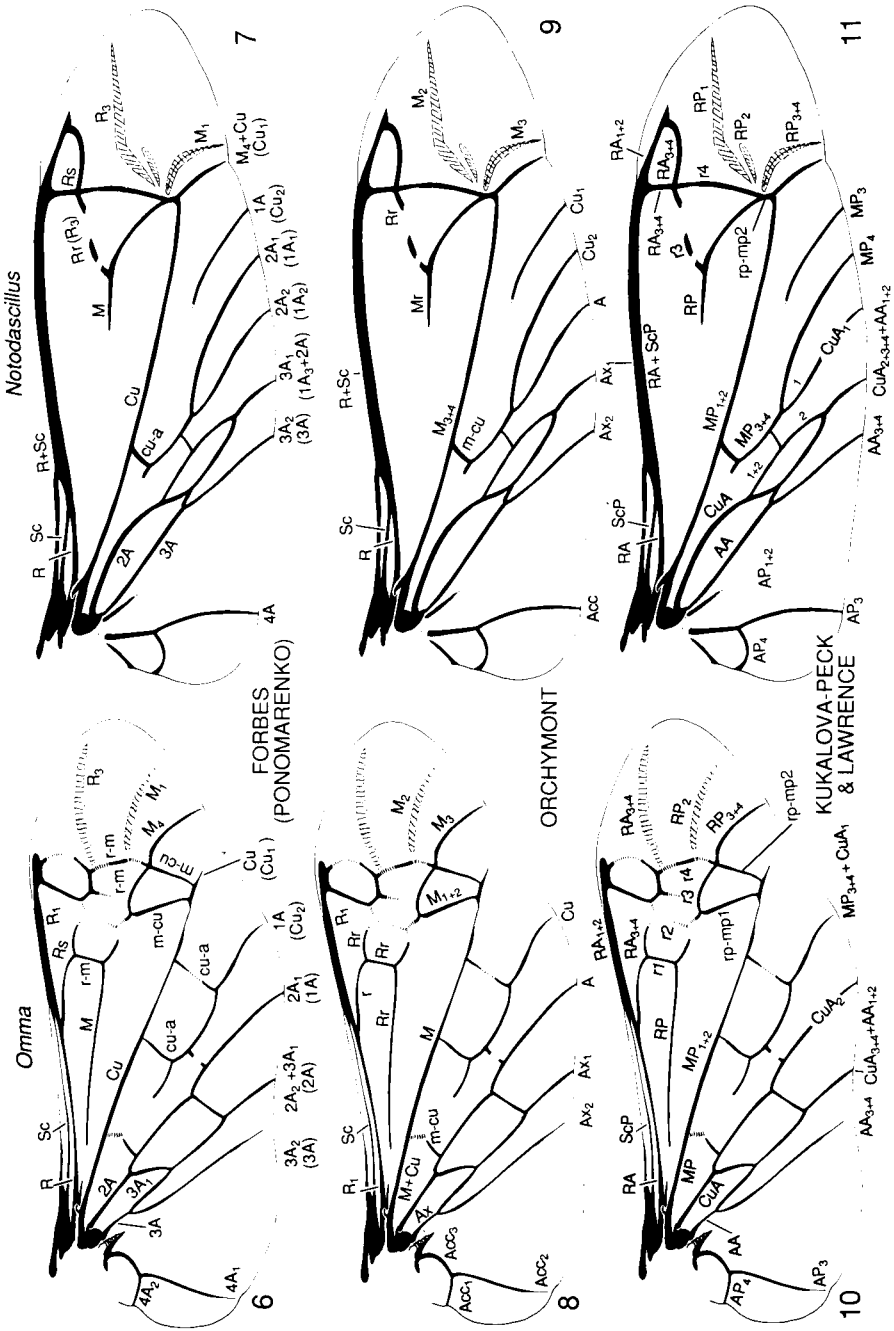
Figs. 6-11. Comparison of the venational schemes used by Forbes and Ponomarenko (6, 7), by d'Orchymont (8, 9), and in the present paper (10, 11) for an archostematan [ Omma stanleyi Newman (6, 8, 10)] and a polyphagan [ Notodascillus sublineatus Carter (7, 9, 11)] wing. In Figures 6 and 7, the names used by Ponomarenko are in parentheses.
