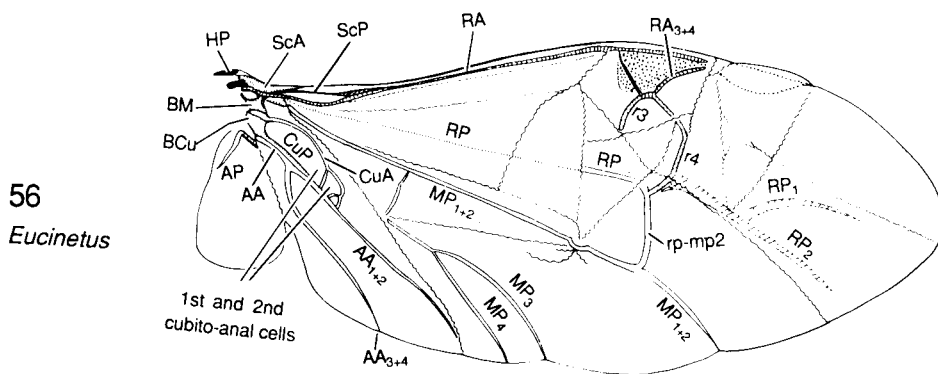
Figs. 54-56. Eucineoidea: 54, Pseudomicrocara sp. (Scirtidae); 55, Macrohelodes sp. (Scirtidae); 56, Eucinetus infumatus LeConte (Eucinetidae).
