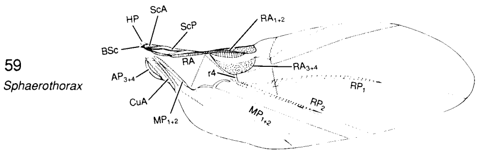
Figs. 57-59. Eucineoidea, Clambidae: 57, Calyptomerus oblongulus Mannerheim; 58, Acalyptomerus sp.; 59, Sphaerotherax tasmani (Blackburn).
