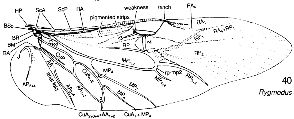
FIGS. 38-40. Staphyliniformia, Hydrophilidae: 38, Pseudohydrobius flavus Lea; 39, Coelostoma sp.; 40, Rygmodus modestus (White).
