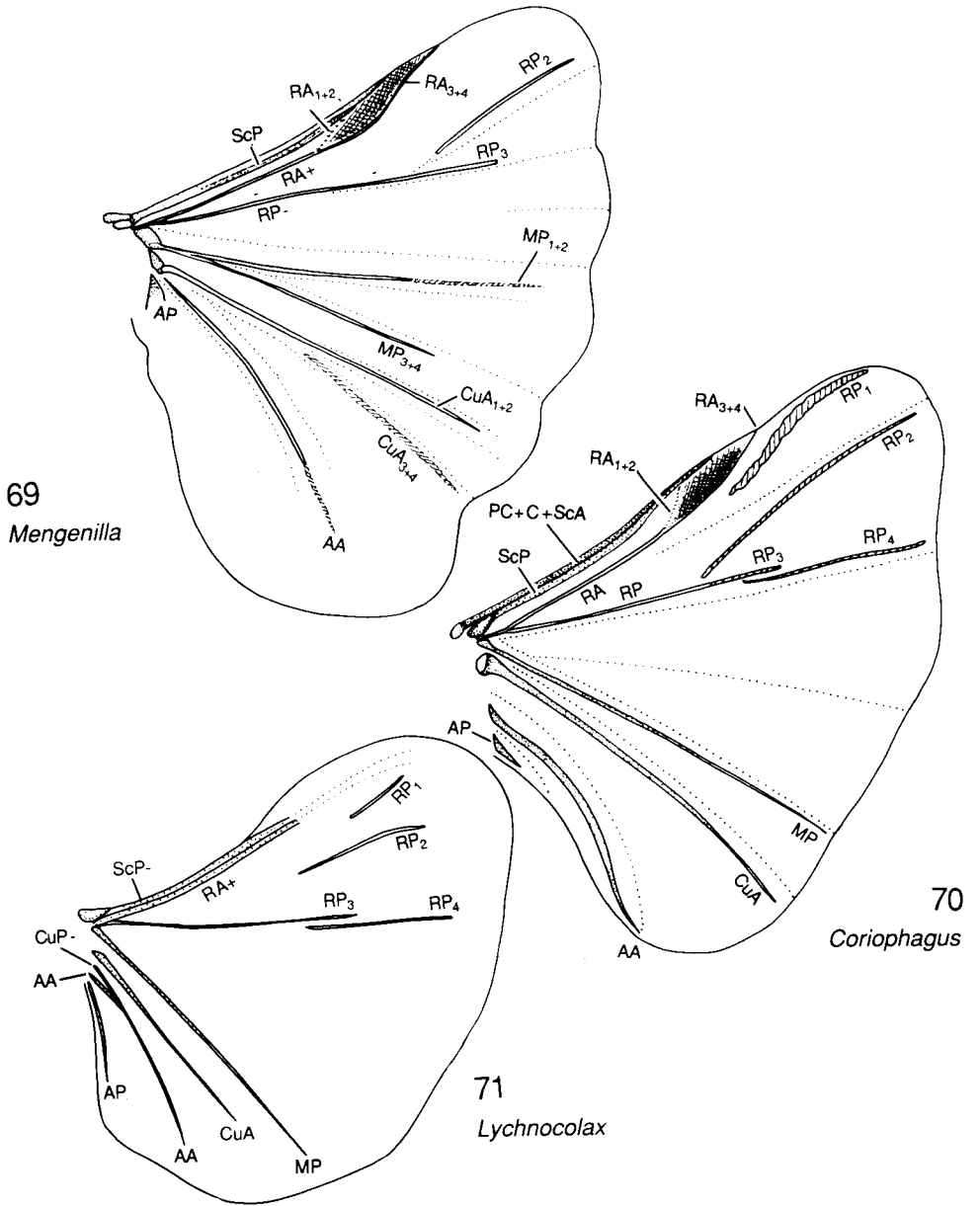
Figs. 69–71. Strepsiptera: 69, Menginilla sp. (Menginillidae); 70, Coriophagus rieki Kinzelbach (Halictophagidae); 71, Lychnocolax sp. (Myrmecolacidae).
