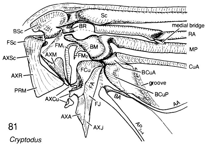
Figs. 80-81. Axillary region and wing base of Scarabaeoidea: 80, Elephastomus proboscideus (Schreibers) (Geotrupidae); 81, Cryptodus paradoxus Macleay (Scarabaeidae).
