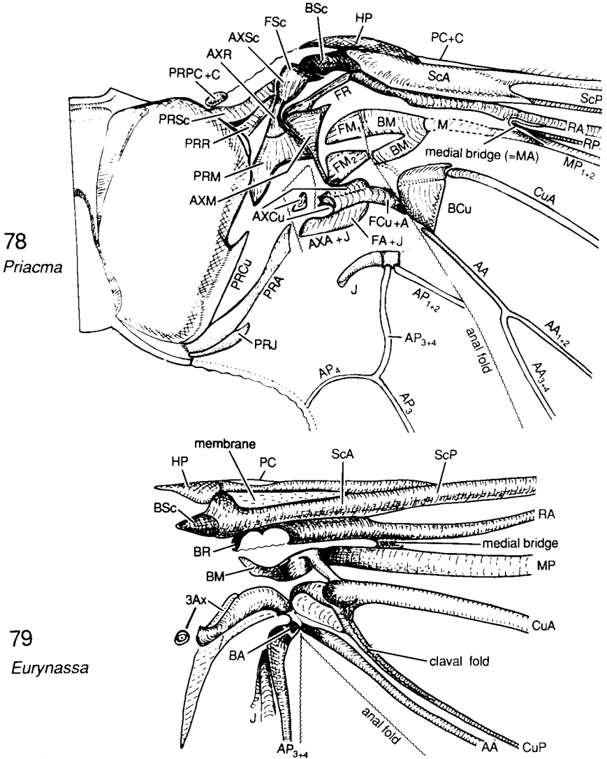
Figs. 78-79. Axillary region and wing base: 78, Archostemata, Priacma serrata LeConte (Cupedidae); 79, Polyphaga, Eurynassa sp. (Cerambycidae).
