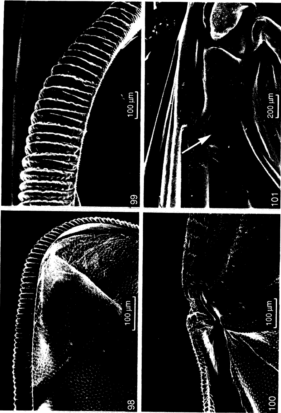
Figs. 98-101. 98-99, radial bar, crimping of radial spring, ventral; 98, Macrogyrus sp.; 99, Calosoma schayeri ; 100, apical hinge, dorsal, Synsdesus cornutus ; 101, portion of wing base showing medial bridge (arrow) and bases of ScA, ScP, R, M, and Cu, Calosoma schayeri .
