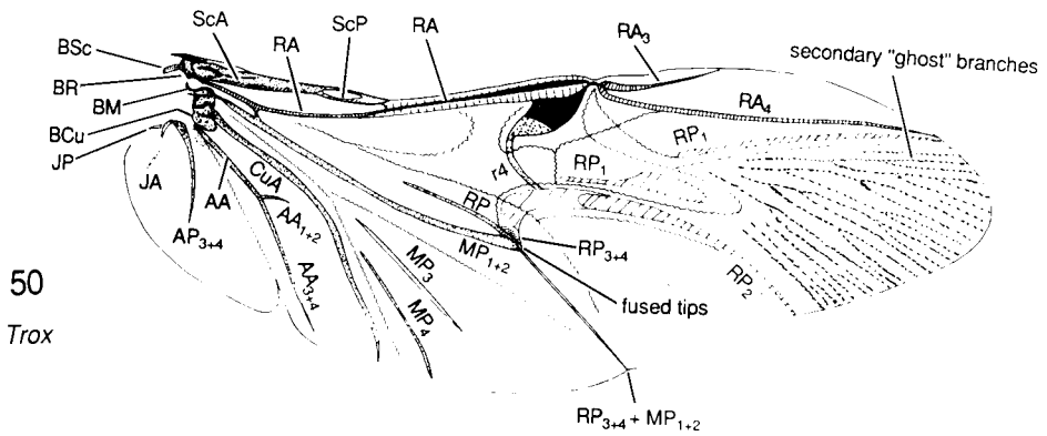
Figs. 48–50. Scarabaeoidea: 48, Glaresis walzae Scholtz (Glaresidae) (male); 49, Glaresis walzae Scholtz (Glaresidae) (female); 50, Trox sp. (Trogidae).
