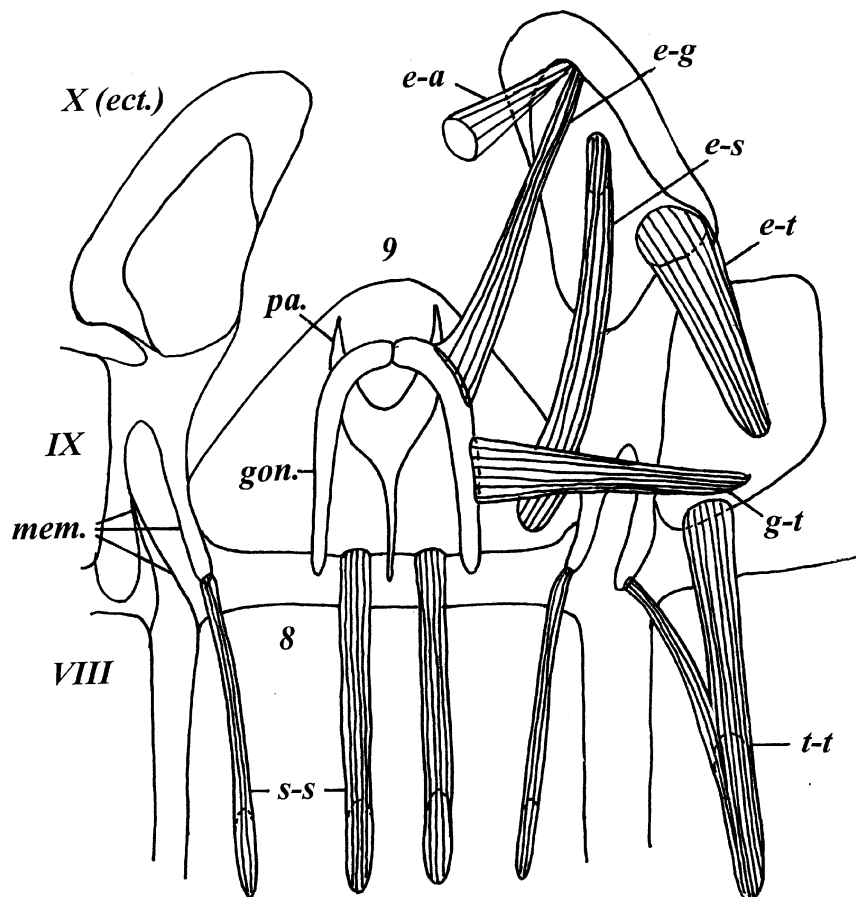
Fig. 9. Internal male genitalia structures of Creoleon plumbeus (for explanation see Fig. 1)
