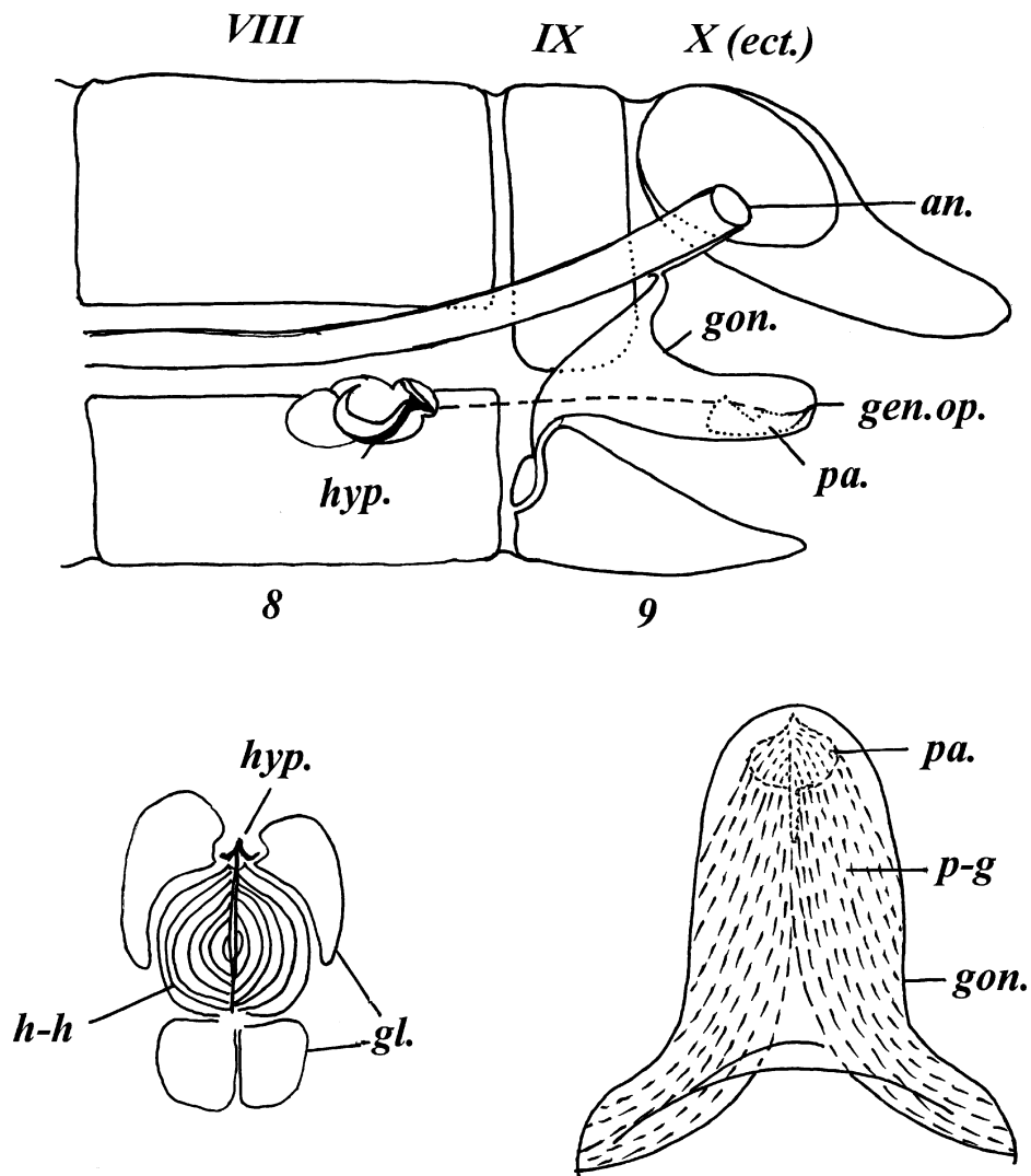
Figs 1–3. Internal male genitalia structures of Myrmecaelurus trigrammus . Explanation of figures: 1, 6 – general structure of internal genitalia, lateral view; 2, 7 – ejaculatory complex, dorsal view; 3, 8 – aedeagal subcomplex, dorsal view; 4, 9 – musculature of the pregenital and copulative complexes, dorsal view; 5 – proctal subcomplex, dorsal view. Structures: VIII–X – abdominal tergites; X (ect.) – ectoproct; 8, 9 – abdominal sternites; an. – anus; gen. op. – genital opening; gl. – glands; gon. – gonarcus; hyp. – hypandrium internum; mem. – membrane; pa. – paramere; pap. – rectal papilla. Muscles: e–a – ectoproct – anus; e–g – ectoproct – gonarcus; e–s – ectoproct – sternite 9; e–t – ectoproct – tergite IX; g–s – gonarcus – sternite 9; g–t – gonarcus – tergite IX; h–h – hypandrium – hypandrium; p–g – paramere – gonarcus; s–s – sternite 8 – sternite 9; t–t – tergite VIII – tergite IX
