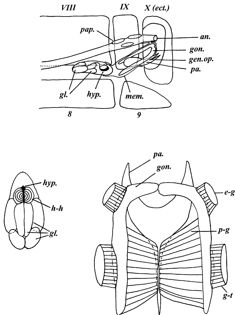
Figs 6–8. Internal male genitalia of Creoleon plumbeus (for explanation see Fig. 1)
