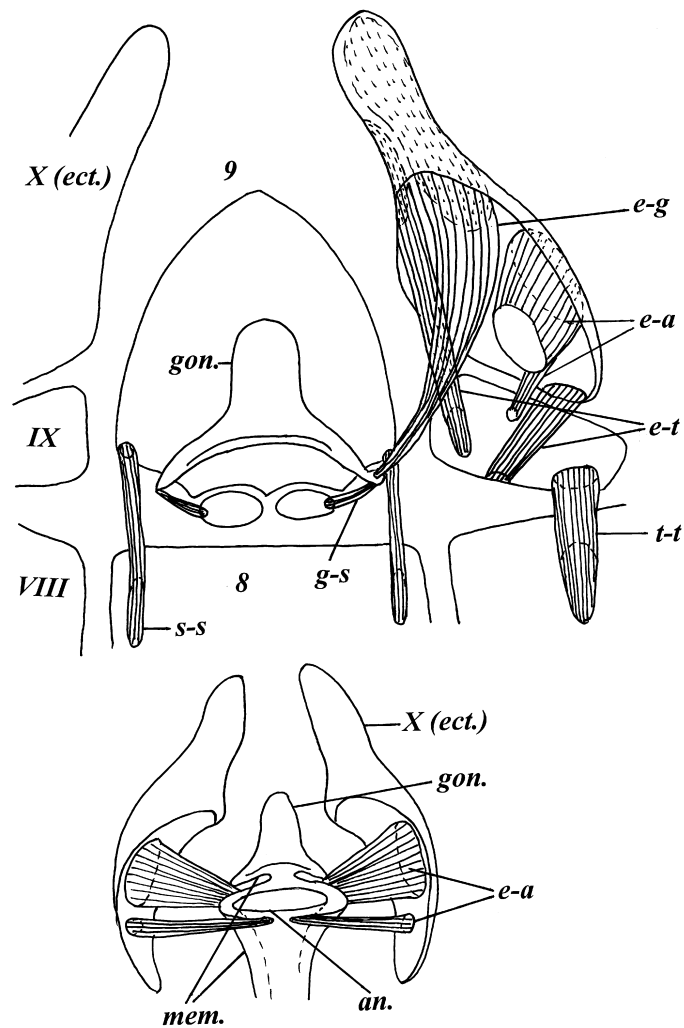
Figs 4–5. Internal male genitalia structures of Myrmecaelurus trigrammus (for explanation see Fig. 1)
