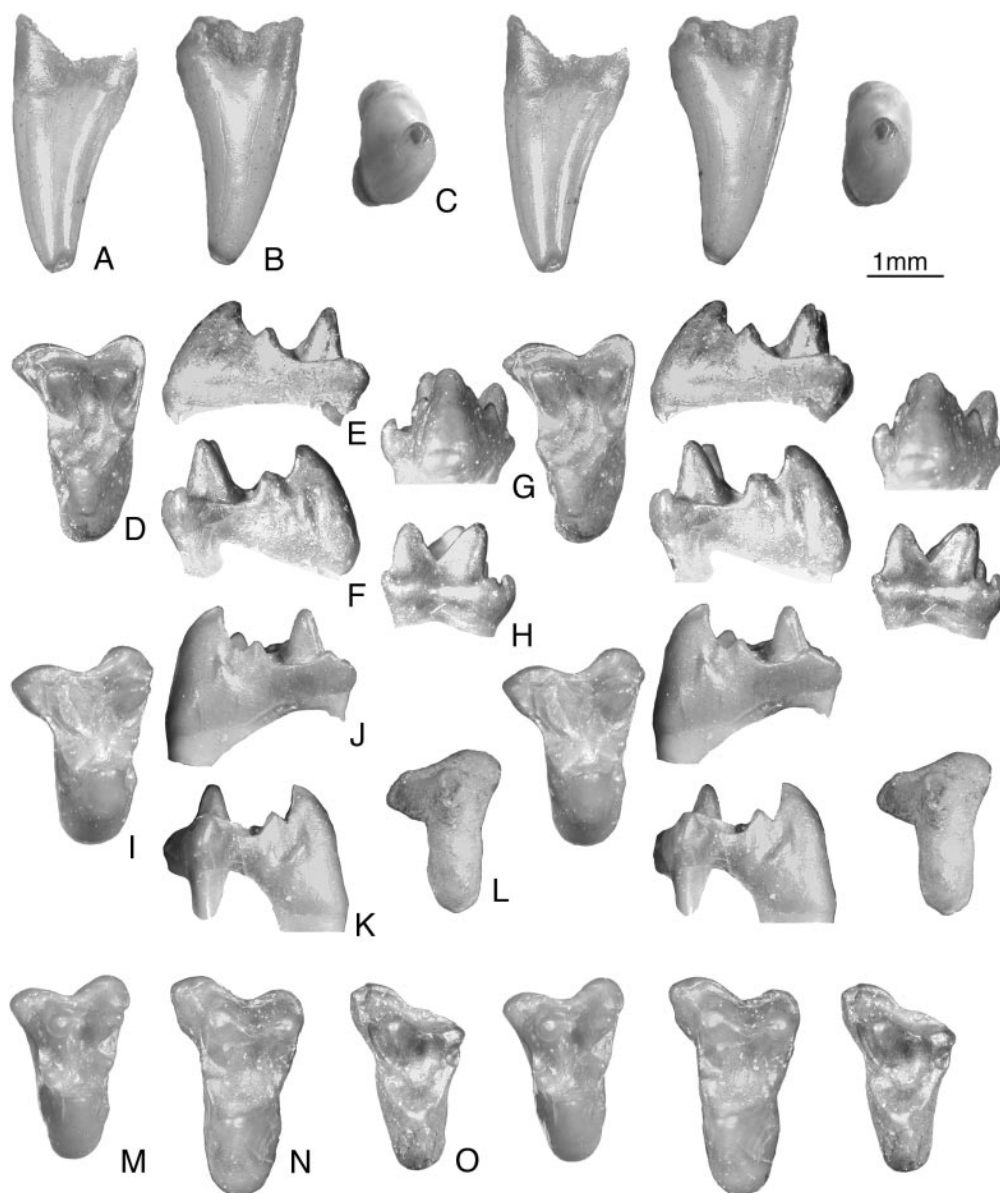
FIGURE 3. Kulbeckia kulbecke , stereophotographs of isolated upper teeth. A , lingual; B , labial; C , occlusal views, ZIN C.82566, right upper canine; D , occlusal; E , posterior; F , anterior; G , lingual; H , labial views, CCMGE 52/12455, left M1 (holotype of K. kulbecke ); I , occlusal; J , anterior; K , posterior views, URBAC 98-134, right M1 (reversed, paracone missing); L , URBAC 98-102, right P5 (reversed, heavily chemically weathered); M , occlusal view, URBAC 98-100, right M1 (reversed); N , occlusal view, ZIN C.82565, left M2; O , occlusal view, CCMGE 54/12455, right M3 (reversed).
