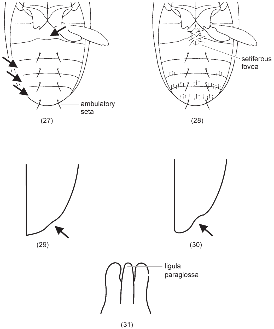
Fig. 27–31 (27–28) Pubescence of venter: (27) paired ambulatory setae only; (28) paired ambulatory setae, numerous short setae, and male setiferous fovea. (29–30) Subapical situation of right elytron: (29) weak; (30) strong. (31) Ligula as long as paraglossae.
