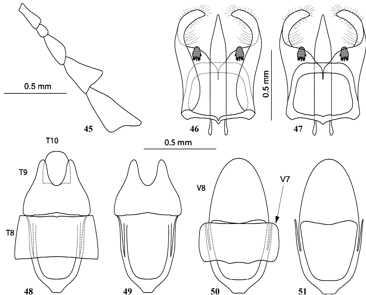
Figs 45–51. Details of Omethidae and Omalisidae: 45–47 — Drilonius flavipennis sp.n., holotype; 48–51 — Omalisus fontisbellaquaei ; 45 — antennomeres 1–5, 46–47 — aedeagus; 48, 50 — genital capsule; 49 — tergite 9; 51 — ventrite 8; 46, 50, 51 — ventrally, 47, 48, 49 — dorsally; T — tergite; V — ventrite [Figs 48–51 after Kazantsev, 2007, modified].
