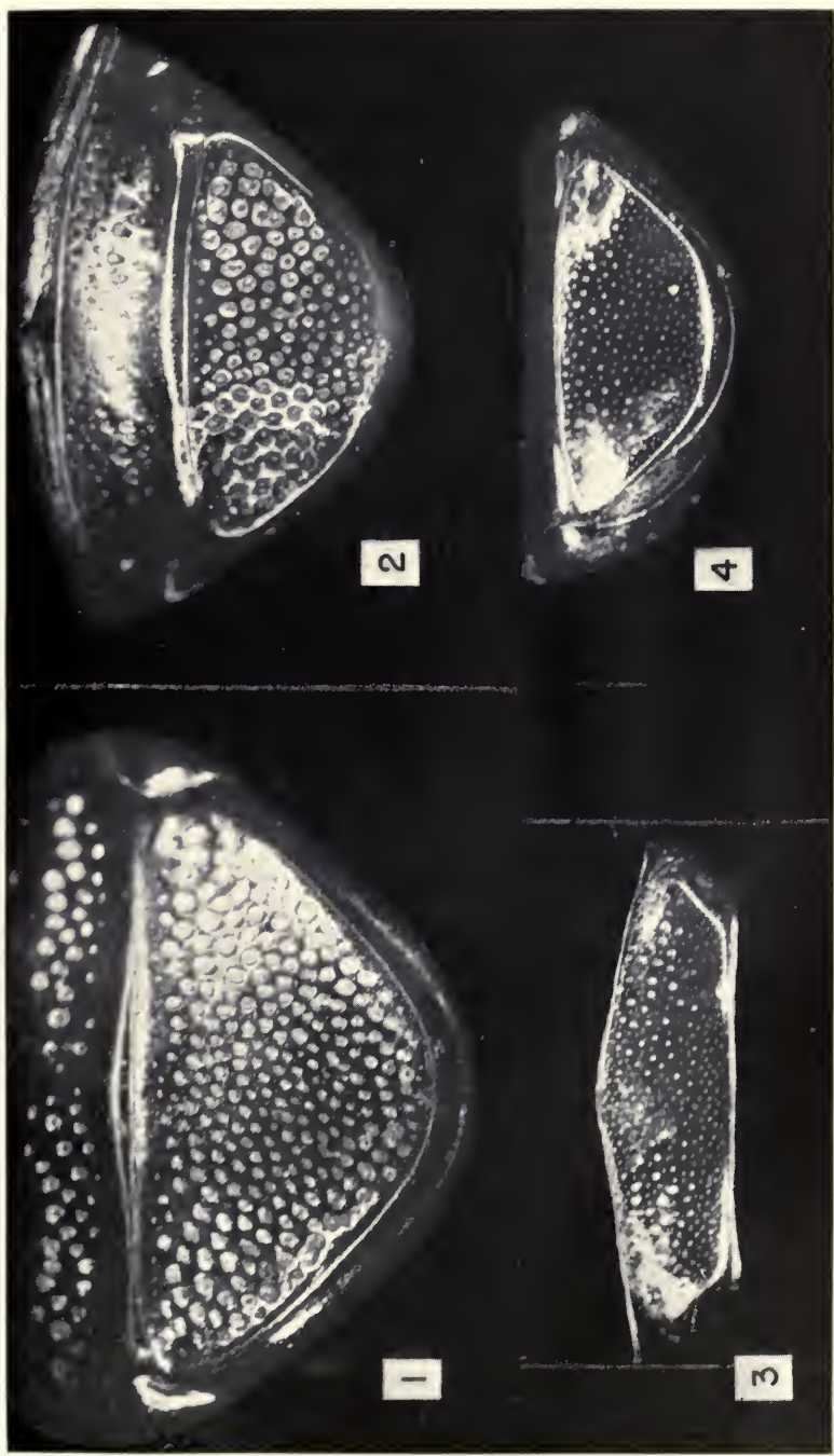
1, Platysoma urvillei Le Guillou, pygidia. 2, P. montrouzieri Fauvel, pygidia. 3 and 4, P. comencum Fauvel, holotype, pygidium and pygidium. \times 43 .
