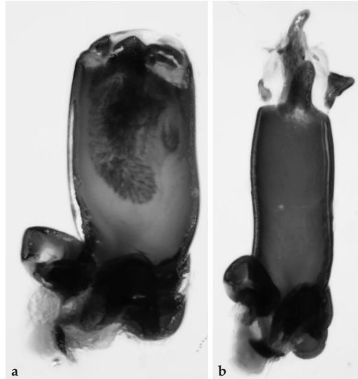
Fig. 15. Aedeagus of Parazuphium species, ventral view: a. P. chevrolatii , b. P. salmoni spec. nov.
