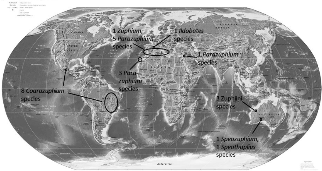
Fig. 18. Distribution of subterranean Zuphiini species.
